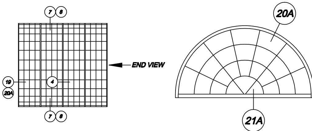
STANDARD 180° VAULT
